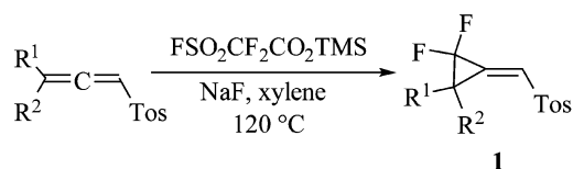
Scheme 1. Synthesis of difluoro(methylene)cyclopropanes (for R 1 , R 2 see Table 2).
