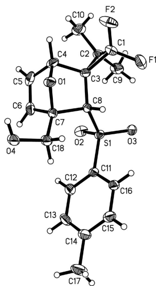
Figure 2. Crystal structure of cycloadduct 2j .
