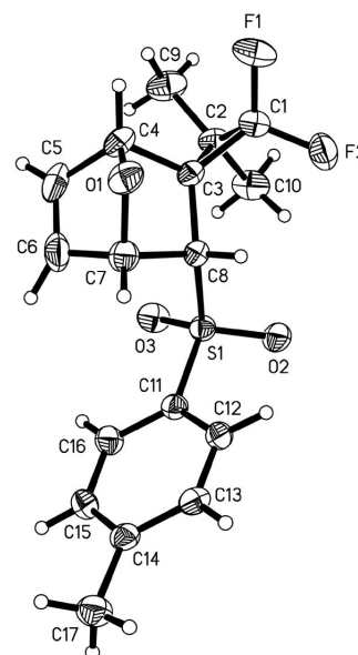
Figure 1. Crystal structure of cycloadduct 2a .
